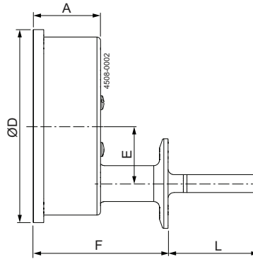
Clamp DN38 (ISO 2852) / Clamp DN40 (DIN32676) TE67Dx1xxx2xxx
