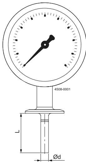
Clamp DN38 (ISO2852) / Clamp DN40 (DIN32676) TE67Dx1xxx1xxx
