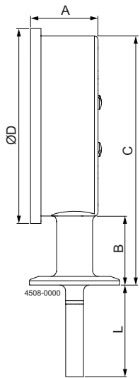
Clamp DN38 (ISO2852) / Clamp DN40 (DIN32676) TE67Dx1xxx1xxx
